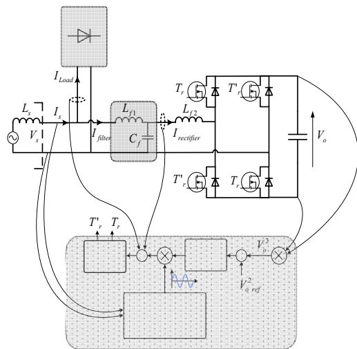
Fig. 2: Mono-phase parallel active power filter structure
