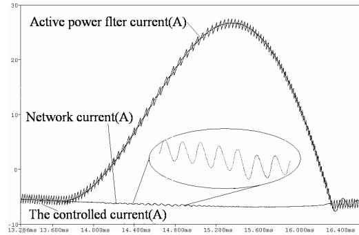
Fig. 11: The behavior of the passive filter
