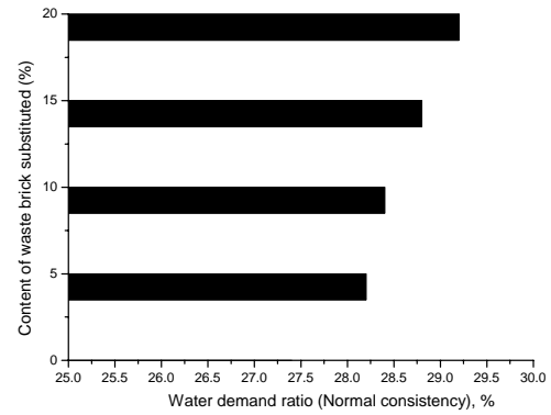
Fig. 2 Variation of the normal consistency cement paste as a function of the content of waste brick
