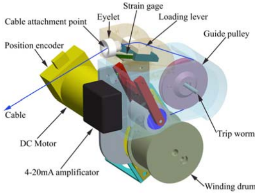
Fig. 3. CAD model of the motorized reel
