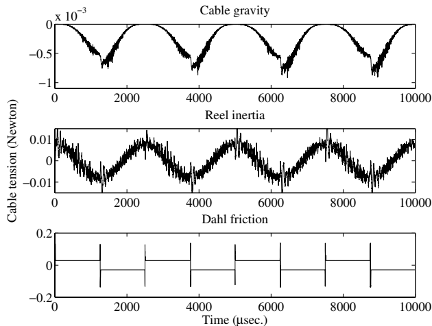
Fig. 15. Force feed-forward compensation with high angular velocity
