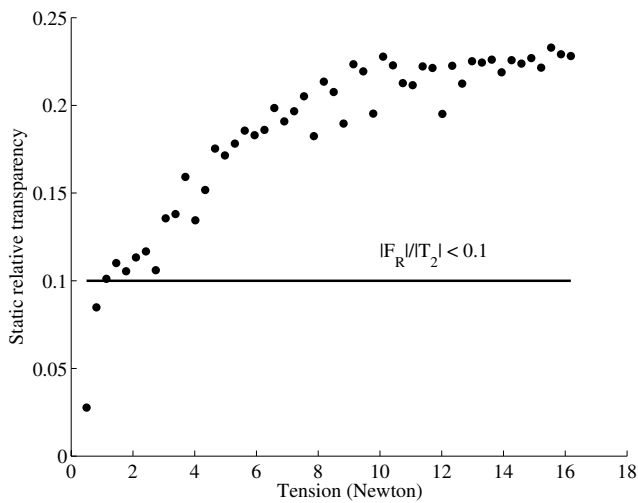
Fig. 6. Evaluation of static transparency
