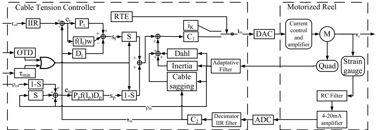
Fig. 7. Cable tension controller
