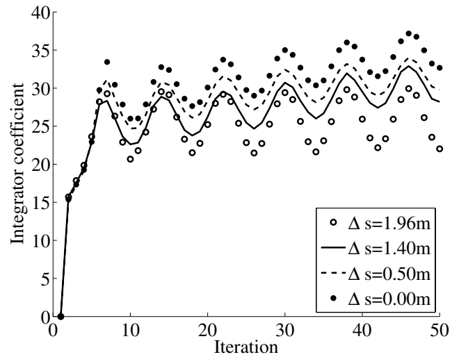
Fig. 12. Evolution of the integrator coefficient
