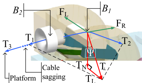
Fig. 4. Cable tensions and friction forces
