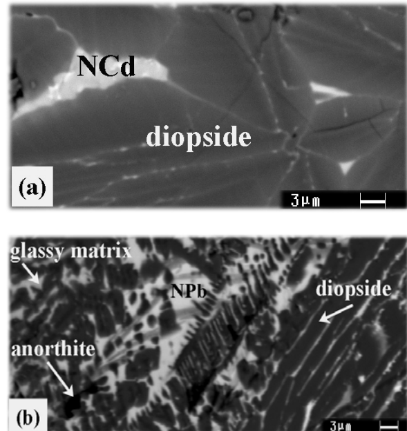
Fig. 1 Scanning Electron Microscope pictures of (a) GD16Cd (Glass-ceramic doped with 16 wt% of CdO) and (b) GD12Pb (Glass-ceramic doped with 12 wt% of PbO)
