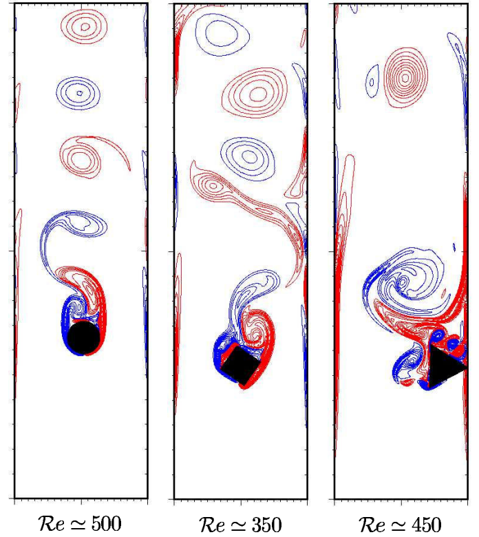
Fig. 3: Vorticity contours for a single particle settling in an infinite channel at Re \in [350 : 500] : effect of particle shape, transition from periodic flow (circular cylinder) to organized chaos (triangle)
