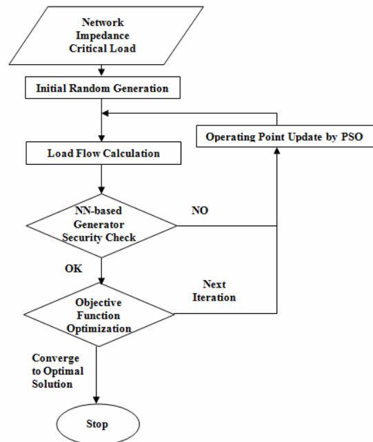
Fig. 5 PSO based OPF Flowchart
