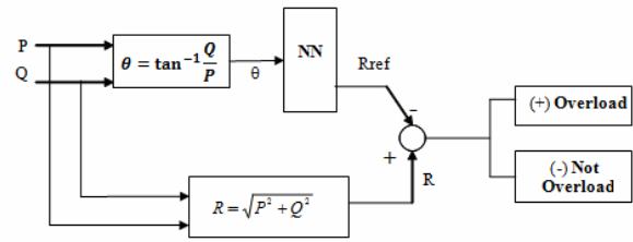
Fig. 4 The security check algorithm
