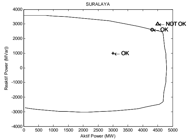
Fig. 8 Generator Security Check
