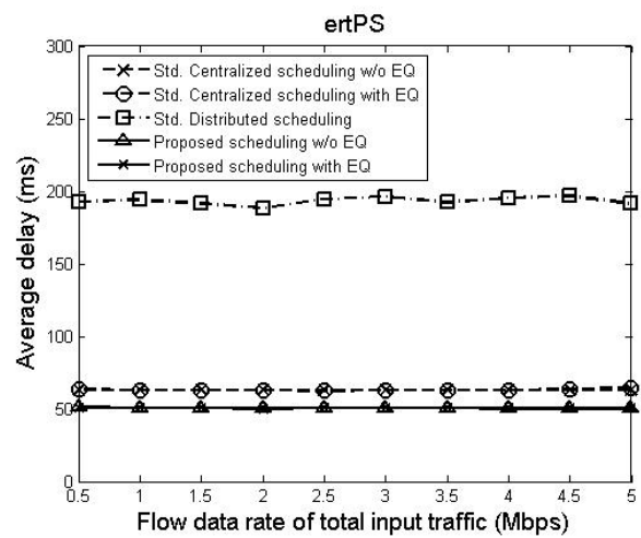
Fig. 8 Average delay of ertPS flows
