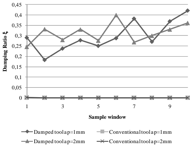
Fig. 10 Damping ratios identified with ARMA(3,2) model
