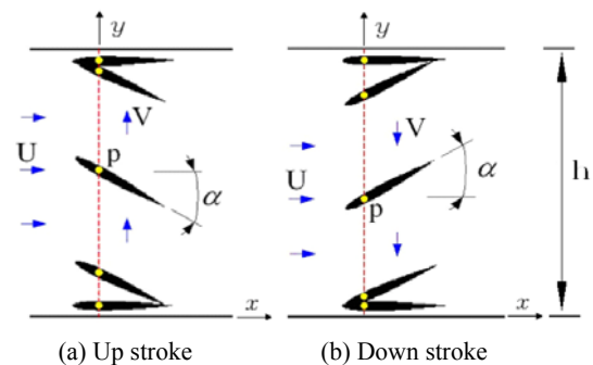
Fig. 1 A model of propulsion mechanism
