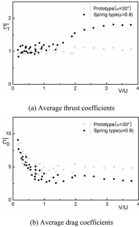
Fig. 8 Average thrust and drag coefficients with velocity ratio
