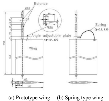
Fig. 3 Structure of the wing and shaft (unit:mm)
