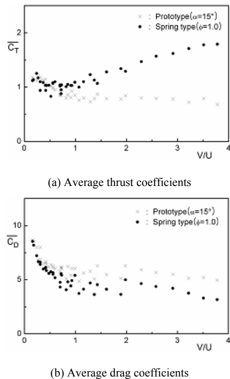
Fig. 7 Average thrust and drag coefficients with velocity
