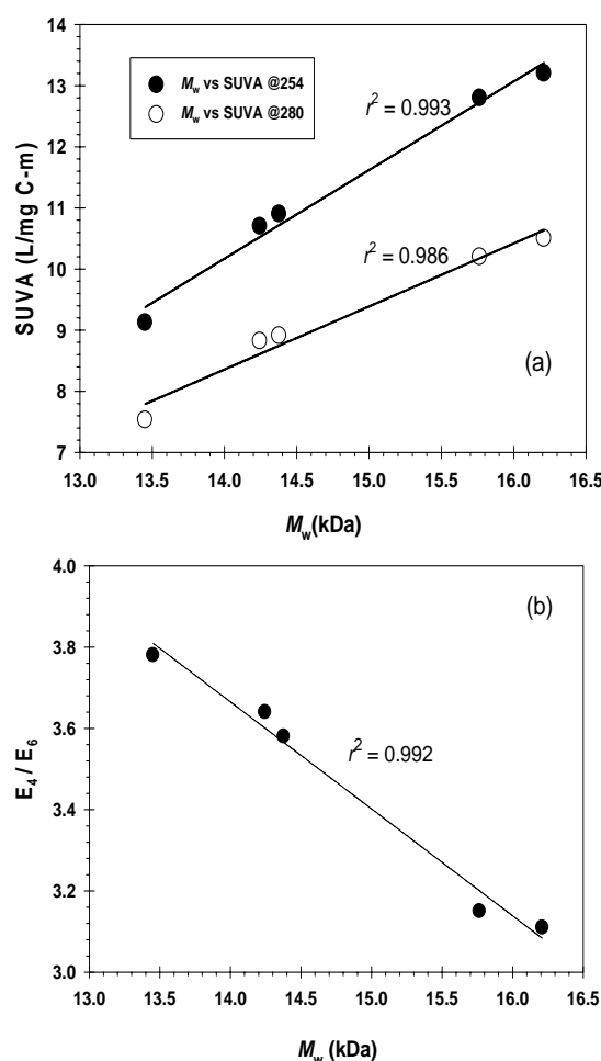
Fig. 4 Relationships between SUVA values at 254 and 280 nm and M w (a), and between E 4 /E 6 and M w (b)
