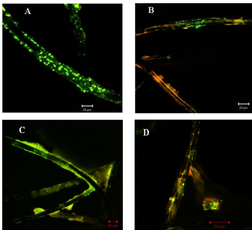
Fig. 6 CLSM of the biofilm developed on the anode in closed-(A and C) and open-(B and D) circuit sediment MFCs operated for approximately 5 months (A and B for Lake Sihwa sediment; C and D for Gongji steam sediment; Red: Gram positive; green: Gram negative)
