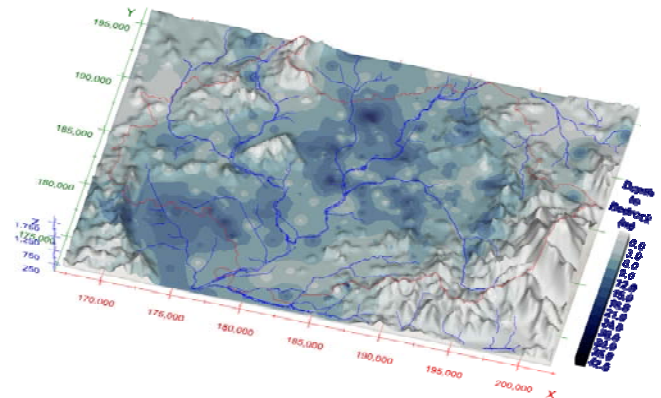
Fig. 5 Spatial distribution of the depth to bedrock
