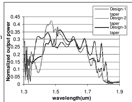
Fig. 12 The transmission spectra for various taper designs.
