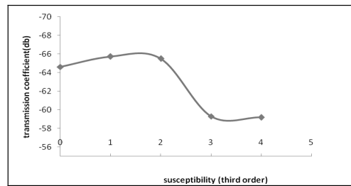
Fig. 7 Transmission coefficient of a nonlinear PhC lattice as a function of the nonlinearity.
