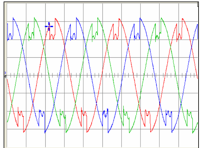
Fig. 10 Three phase voltages in mode 2/3
