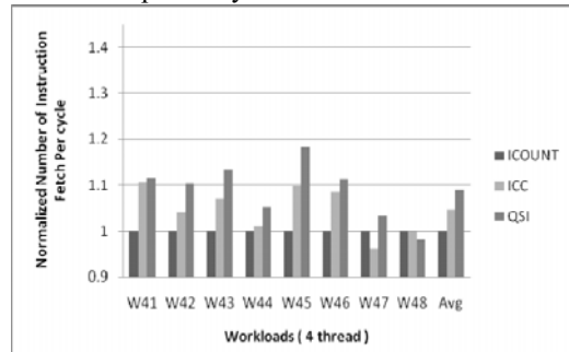
Figure 5. Normalized fetch rate of 4-thread workloads
