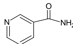
Fig. 1 Chemical structure of nicotinamide
