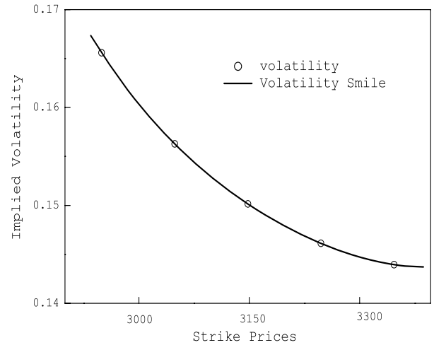
Fig. 5. Volatility smile (smirk) made by a 4-th order polynomial fit of the UGF estimates taken at t=100 .
