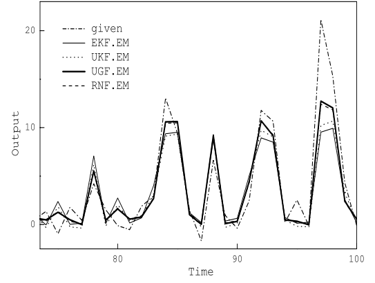
Fig. 1. Approximations of the UNGM series by the studied filters.
