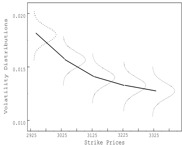
Fig. 6. Volatility distribution smile (smirk) made as piecewise-line of the UGF estimates taken at t=200 .
