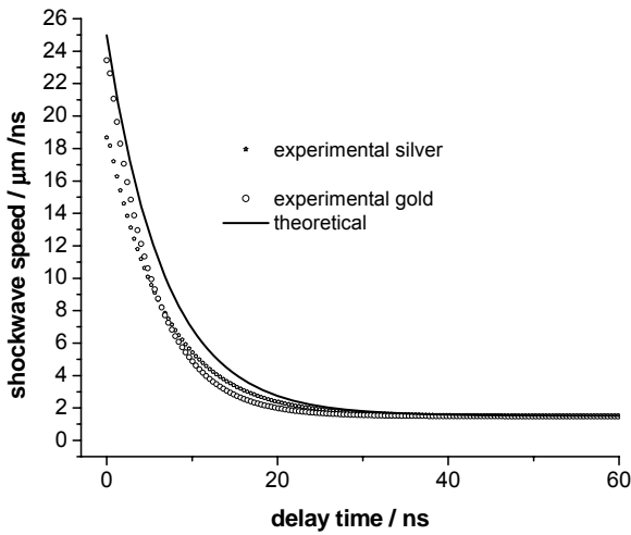
Fig. 3. Speed dynamics of shock wave in water
