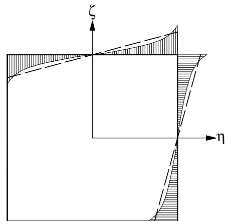
Fig. 14 Warping stresses distribution
