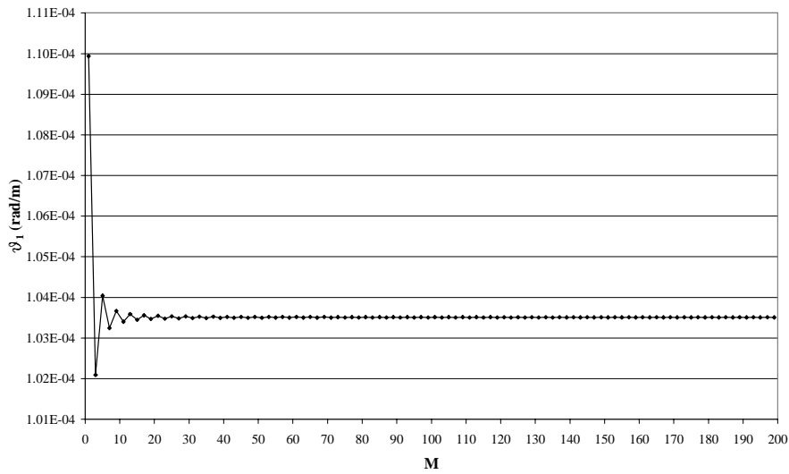
Fig. 4 Unit twist angle convergence x = 1.8 m
