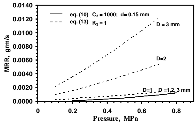
Fig. 12 Effect of pressure on material removal rate at different nozzle diameters for the two models \{\rho_a = 2.3 \text{ g/cm}^3; P = 0.5 \text{ MPa}; \eta = 0.7 and \sigma_{fw} = 5000 \text{ MPa} for glass}
