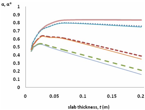
Fig. 6 True energy storage density factor, \alpha and \alpha^* versus slab thickness, t (m)
