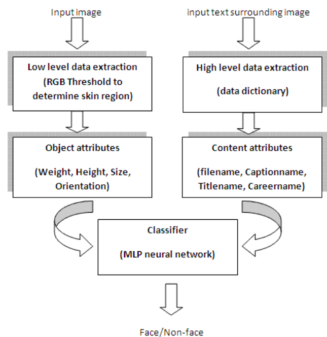
Fig. 1 The experimental procedure
