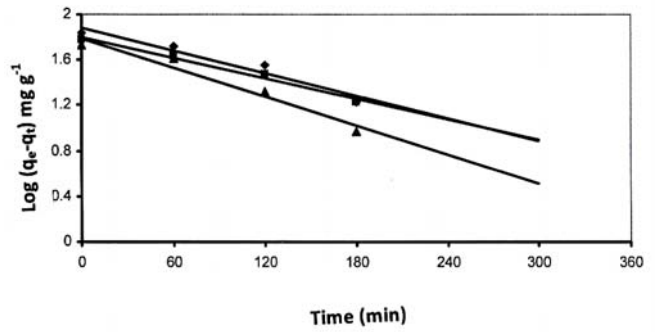
Fig. 2 Plots of pseudo first order kinetics of the interaction between Copper(II) and teak leaves powder dosage at 293 K (♦) D = 0.3 g.l -1 , D = (■) 0.4 g.l -1 , D = (▲) 0.5 g.l -1
