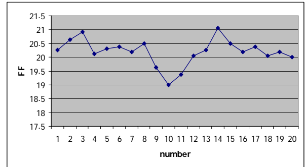
Fig. 3 Moving average control chart for Fill Factor
