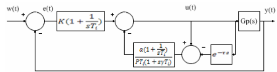
Fig. 8 Another type of structure for PIP controller
