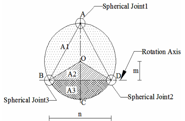
Fig. 2 Schematic representation of moving platform
