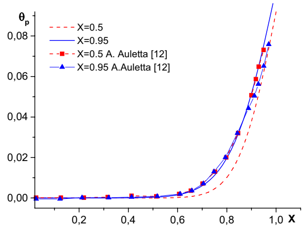
Fig.2. Temperature profiles for the configuration with H/2e=2 . and \Phi = 450 W. Natural convection flow Comparison with experiments.
