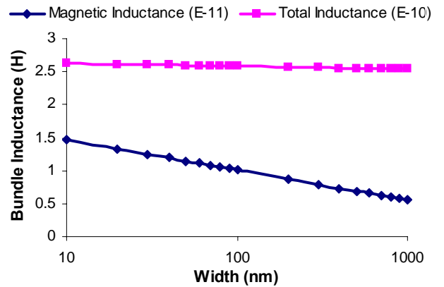
Fig. 3 Inductance Vs bundle width (W)
