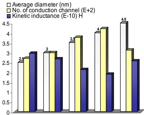
Fig. 5 Kinetic inductance Vs Average diameters
