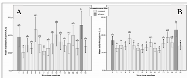
Fig. 3. A) Mean midday light levels (left) and B) mean daily light levels (photosynthetically active radiation; \mu mol m^{-2} s^{-1} ) (right) for all plots (presence of greenhouse film is indicated with light bar shading). Error bars represent 95% confidence intervals. Letters indicate statistical grouping based on two ANOVAs (midday light levels and mean daily light levels) with post-hoc Scheffé tests.
