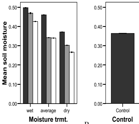
A. B. Fig. 2. A) Soil moisture ( m^3/m^3 VWC) by moisture treatment (shading of bars represent temperature treatment; black = 0 °C, grey = 2.5 °C, white = 5 °C). Error bars represent 95% confidence intervals. B) Control represent plots without rain exclusion structures.
