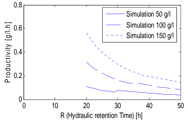
Fig. 5 Effect of hydraulic retention time on the ethanol productivity
