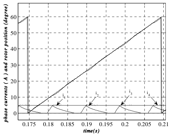
Fig. 10 Phase currents and rotor position
