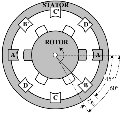
Fig. 1 Cross section of 8/6 poles SRM
