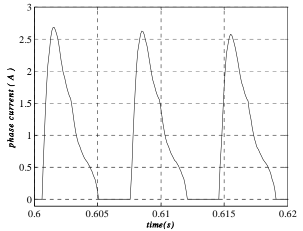
Fig. 9 Phase current for 30 rad/s
