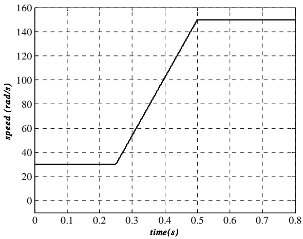
Fig. 5 Rotor speed
