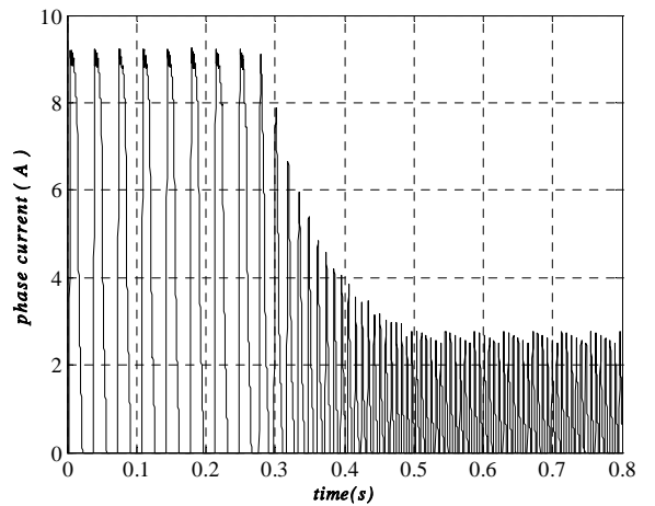
Fig. 4 Phase current for 30-150 rad/s
