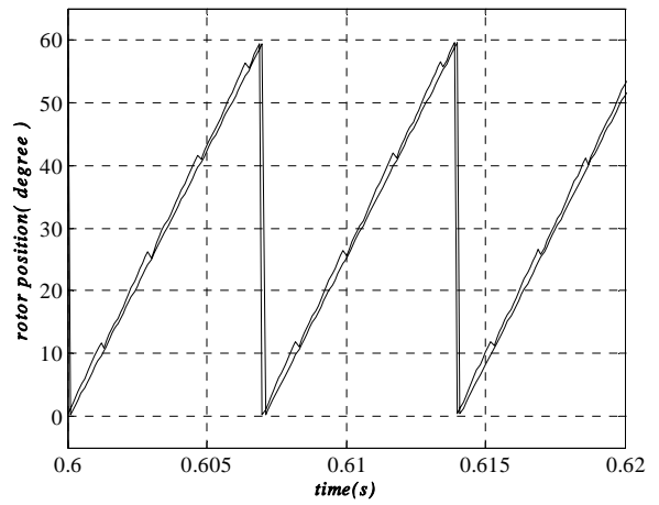
Fig. 8 Actual and desired rotor position for 150 rad/s
