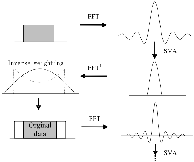
Fig. 1 The flow chart of super-SVA
