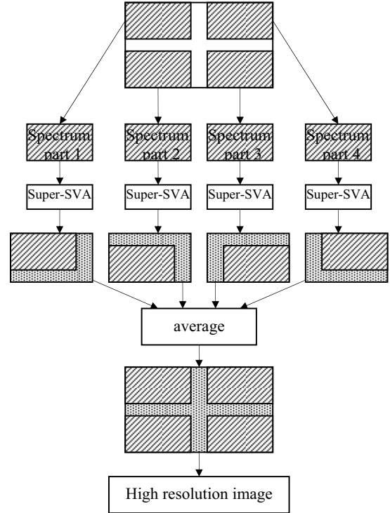
Fig. 2 Super-SVA gap filling procedure
