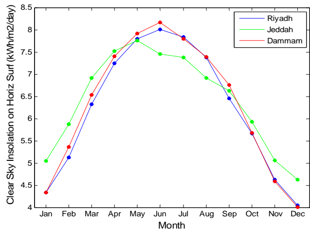
Fig. 2 (c) Monthly average clear sky insolation incident on a horizontal surface
