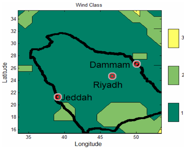
Fig. 6 (b) Wind class 10 m above ground
