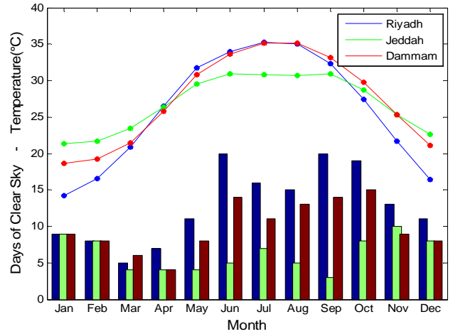
Fig. 2 (a) Monthly average number of clear sky days and average temperature at 10 m above the surface of earth
