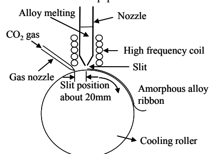
Fig. 1 Scheme diagram of single-roller rapid solidification technique
