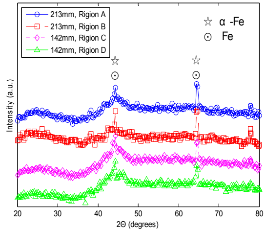
Fig. 5 XRD measured results of different ribbon samples
