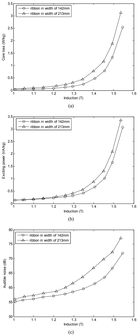
Fig. 9 Measured results of 3-phase 2MVA amorphous-cored transformers: (a) core loss, (b) exciting power, (c) audible noise
