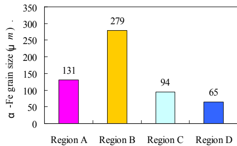
Fig. 6 The grain sizes of the \alpha -Fe for amorphous ribbons, annealing at 350^\circ\text{C} , 2h
