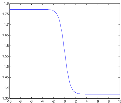
Fig 1 (b) Phase angle \theta vs the argument of the tanh function
