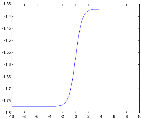
Fig. 1(a) Phase angle \theta vs the argument of the tanh function
