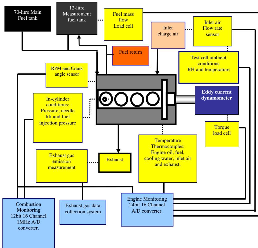
Fig. 1 Experimental setup
