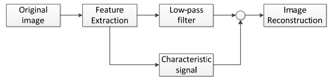
Fig. 1 Block diagram of wavelet de-noising
