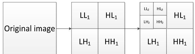
Fig. 2 wavelet decomposition
