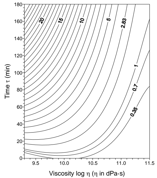
Fig. 5 Map of deflection as a function of viscosity and time
