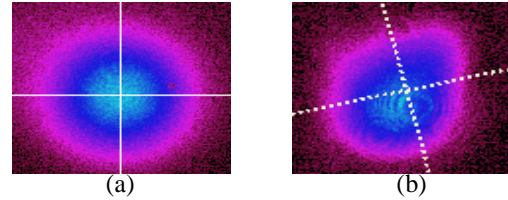
Fig. 3 (a) Near field and (b) Far field of TEM00 mode, r=0.44mm, z=7.9mm
