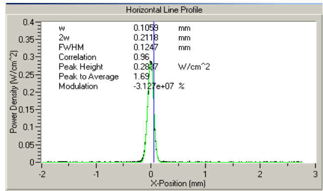
Fig. 12 power density of Gaussian beam with 96% correlation
