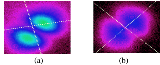
Fig. 4 (a) Near field and (b) Far field of TEM01 mode, r=0.89 mm, z=7.7 mm
