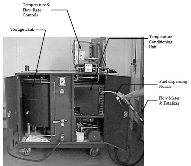
Fig. 4 The fuel-conditioning cart
