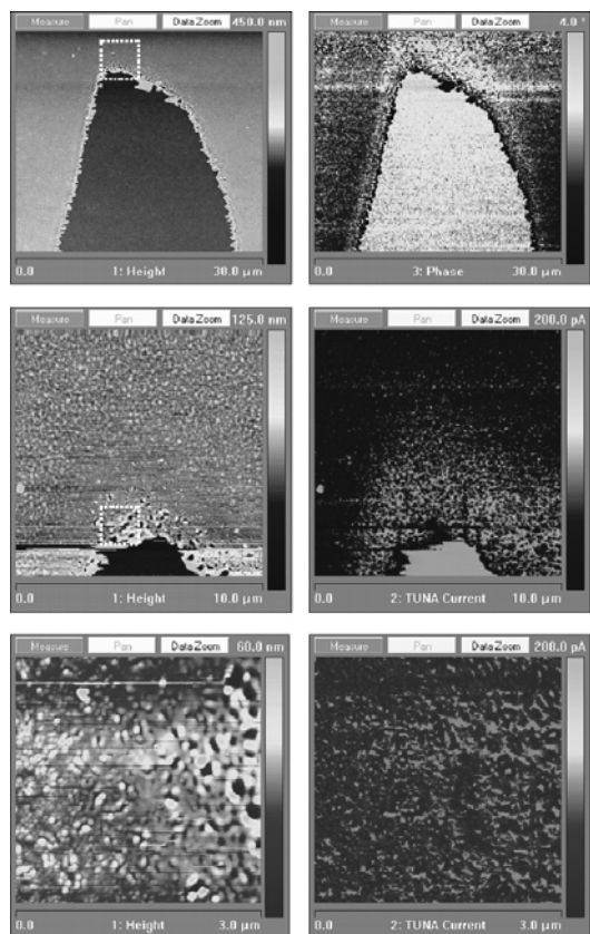
Fig. 6 Analysis of the gold-covered-PMMA by AFM microscope: Top - scaled-up edge of footprint in AFM tapping mode, height (Left) and phase (Right) images, Middle and Bottom- scaled-up edge of footprint in AFM extended TUNA mode, height (Left) and TUNA current (Right) images.
