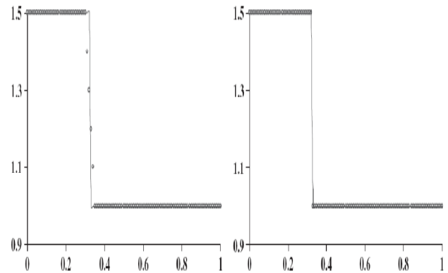
Fig. 3 Solution of Example 2 using third-order scheme (left) and hybrid scheme (right) at t=0.15
