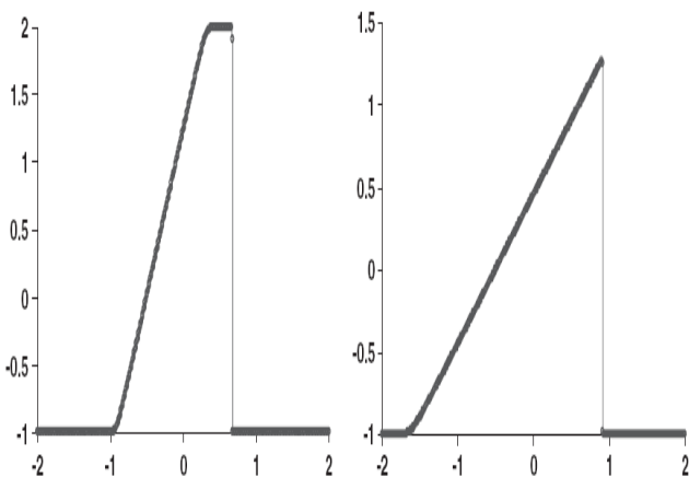
Fig. 2 Solution of Example 1 using the hybrid scheme at t=0.4 (left) and t=1.1 (right).
