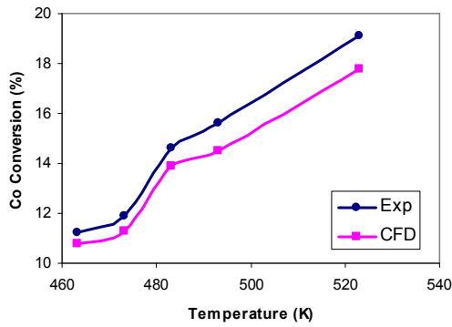
Fig. 2 Carbon monoxide conversion as a function of temperature
