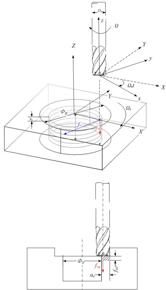
Fig. 1 Kinemics of helical milling
