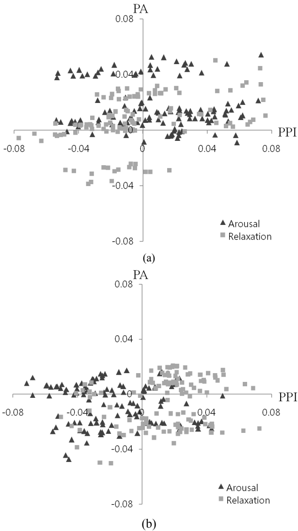
Fig. 4 PPI-PA distribution of 2 subjects for arousal and relaxation (a) Subject 1 (b) Subject 2
