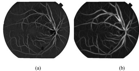
Fig. 3. Maximum modulus response of Gabor wavelet transform over 18 Gabor filters with \varepsilon = 4 and \mathbf{k}_0 = [0, 3] . (a) Scale value of a = 2 pixels. (b) Scale value of a = 5 pixels.
