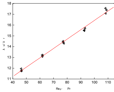
Fig. 7 Relationship between \lambda_b and Re_p \cdot Pr
