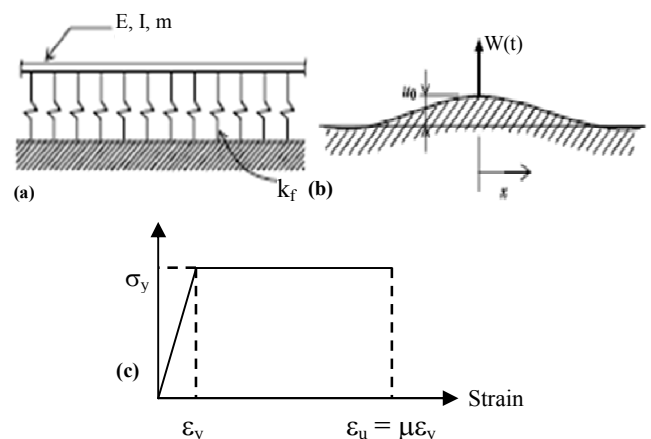
Fig. 1 Beam on elastic foundation model of the pipeline (a), applied blast force (b), assumed material characteristics (c)
