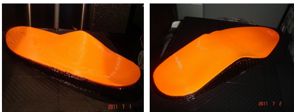
Fig. 8 Manufacturing corrective insoles using rapid prototyping method (flat foot-left, hollow foot-right)
