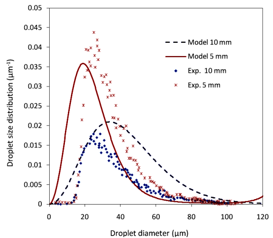
Fig. 4 Droplet size distribution of PWC nozzle for two different positions in downstream direction. Experiment result [16, 31] Reg=11420, Lb=4 mm, D30=45 Micron
